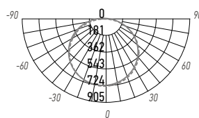
PP0-02 600 PRISMA 18W
