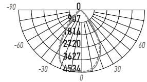
PTR 2260 3S 60W
