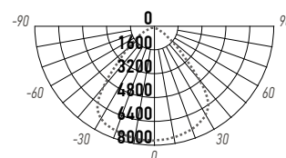
PHB NLO 10 150W
