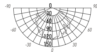
PPG T8i-900 AGRO 12W
