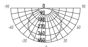
PLED DL7 12W
